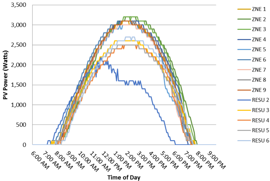
Figure 63: Solar PV Generation (July 22, 2014)
