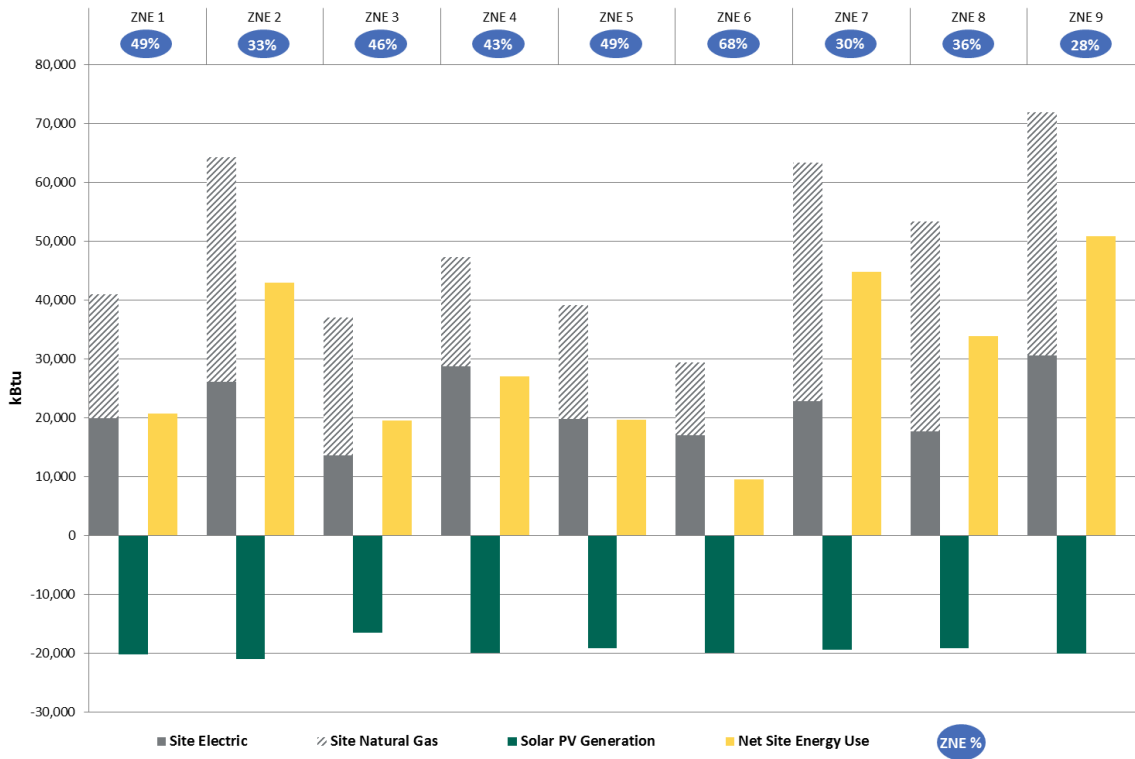
Figure 38: ZNE Site Energy Status for ZNE Block Homes (November 1, 2013 to October 31, 2014)
