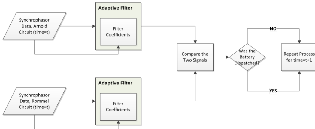
Figure 84: Overall Solution Method II
