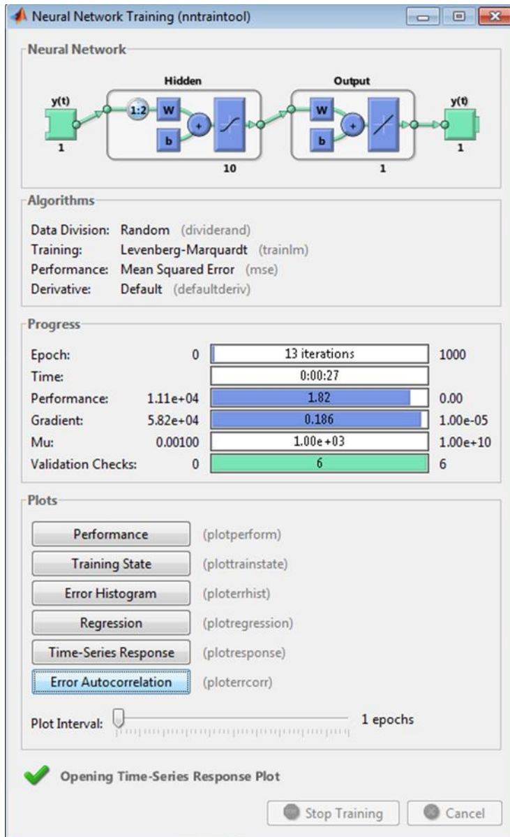
Figure 79: Neural Network Training Summary
