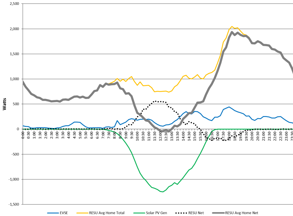
Figure 26: RESU Block Average Home Load Profile (Daily Average for December 2013)
