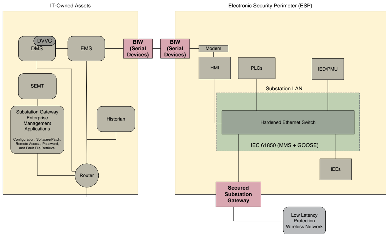
Figure 12: SA-3 Network Architecture
