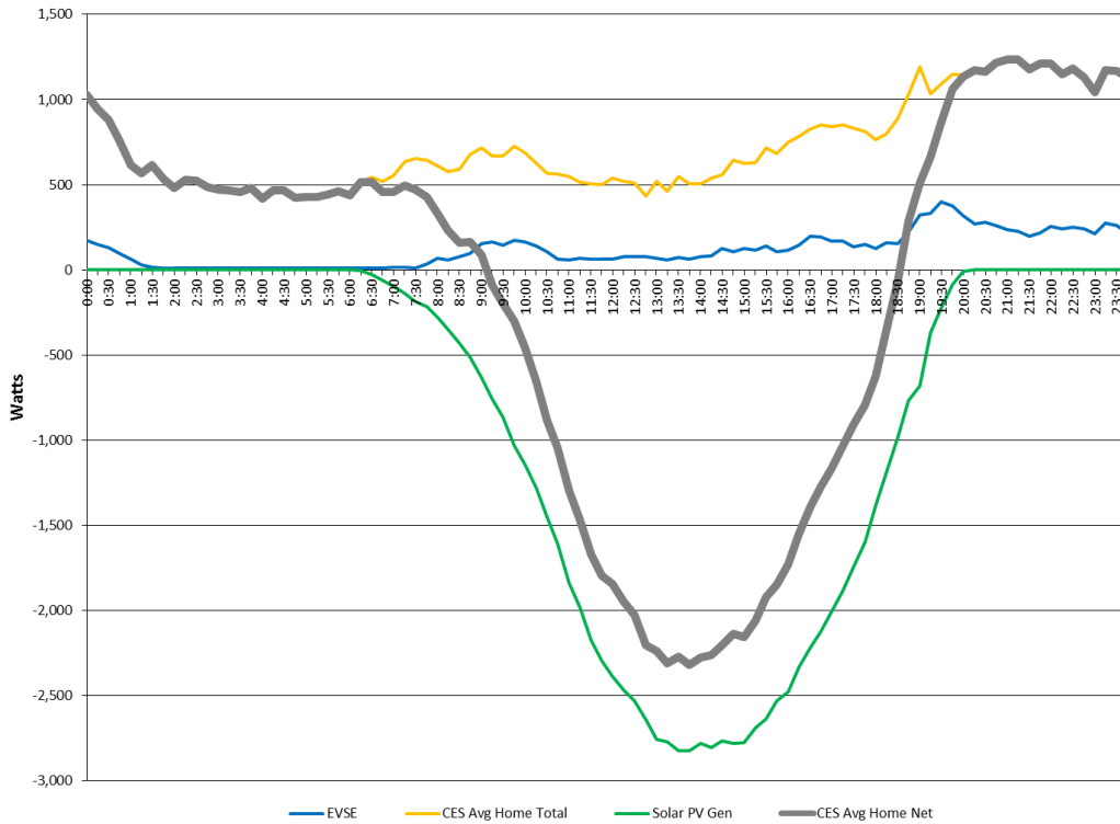
Figure 33: CES Block Average Home Load Profile (Daily Average for June 2014)
