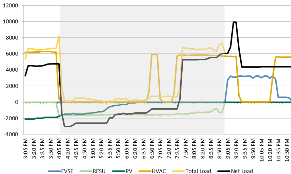
Figure 48: RESU 5 Load Summary (September 15, 2014)
