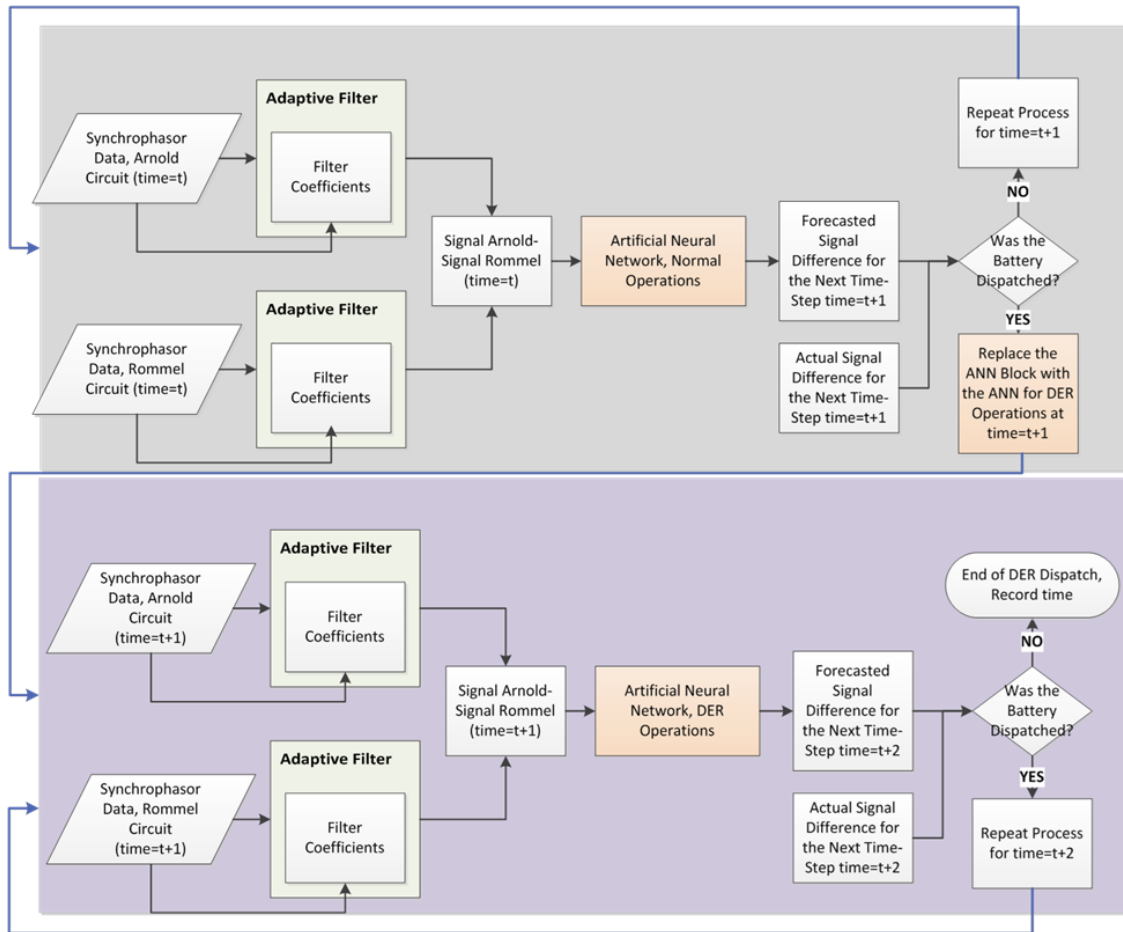
Figure 85: Overall Solution Method III
