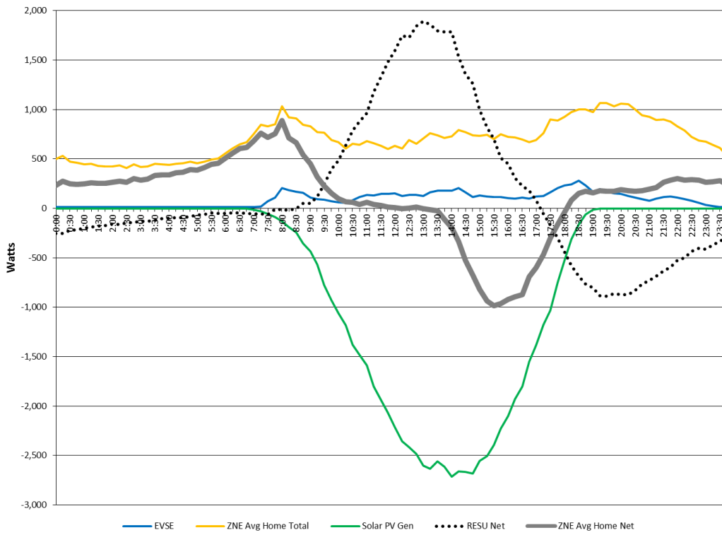
Figure 29: RESU Block Average Home Load Profile (Daily Average for March 2014)
