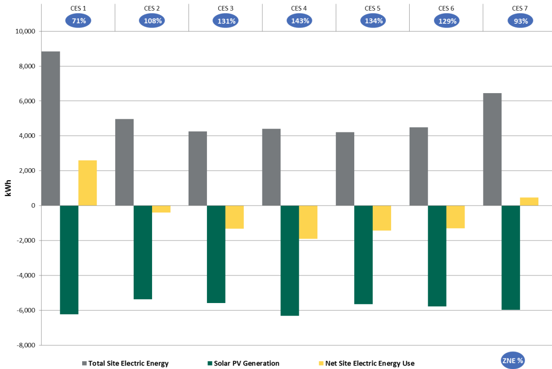
Figure 43: ZNE Site Electric Energy Status for CES Block Homes (November 1, 2013 to October 31, 2014)
