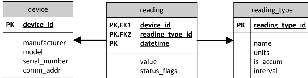
Figure 72: Reference Model Example
