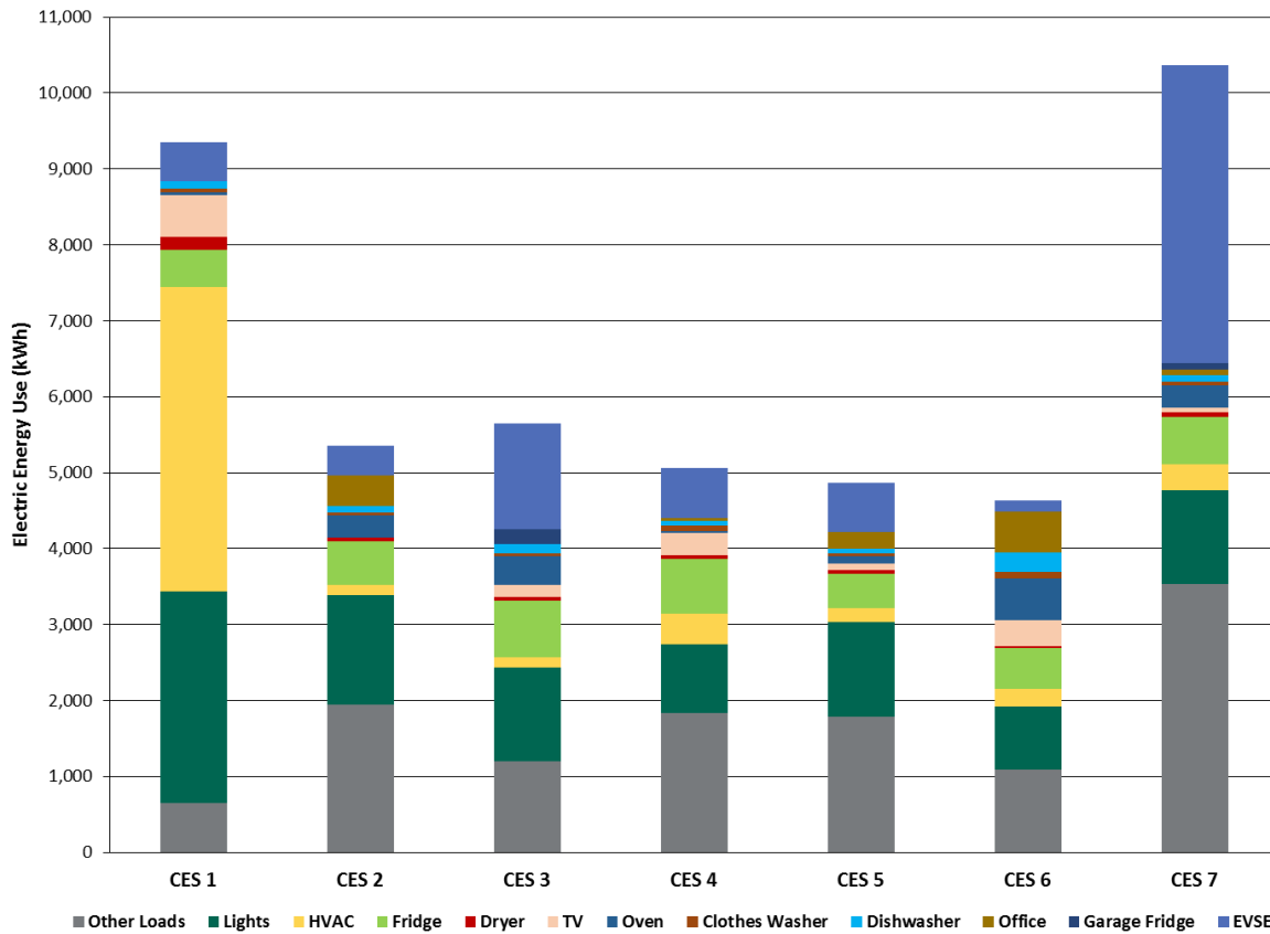
Figure 15: CES Block Electric Energy Use Breakdown (November 1, 2013 to October 31, 2014)
