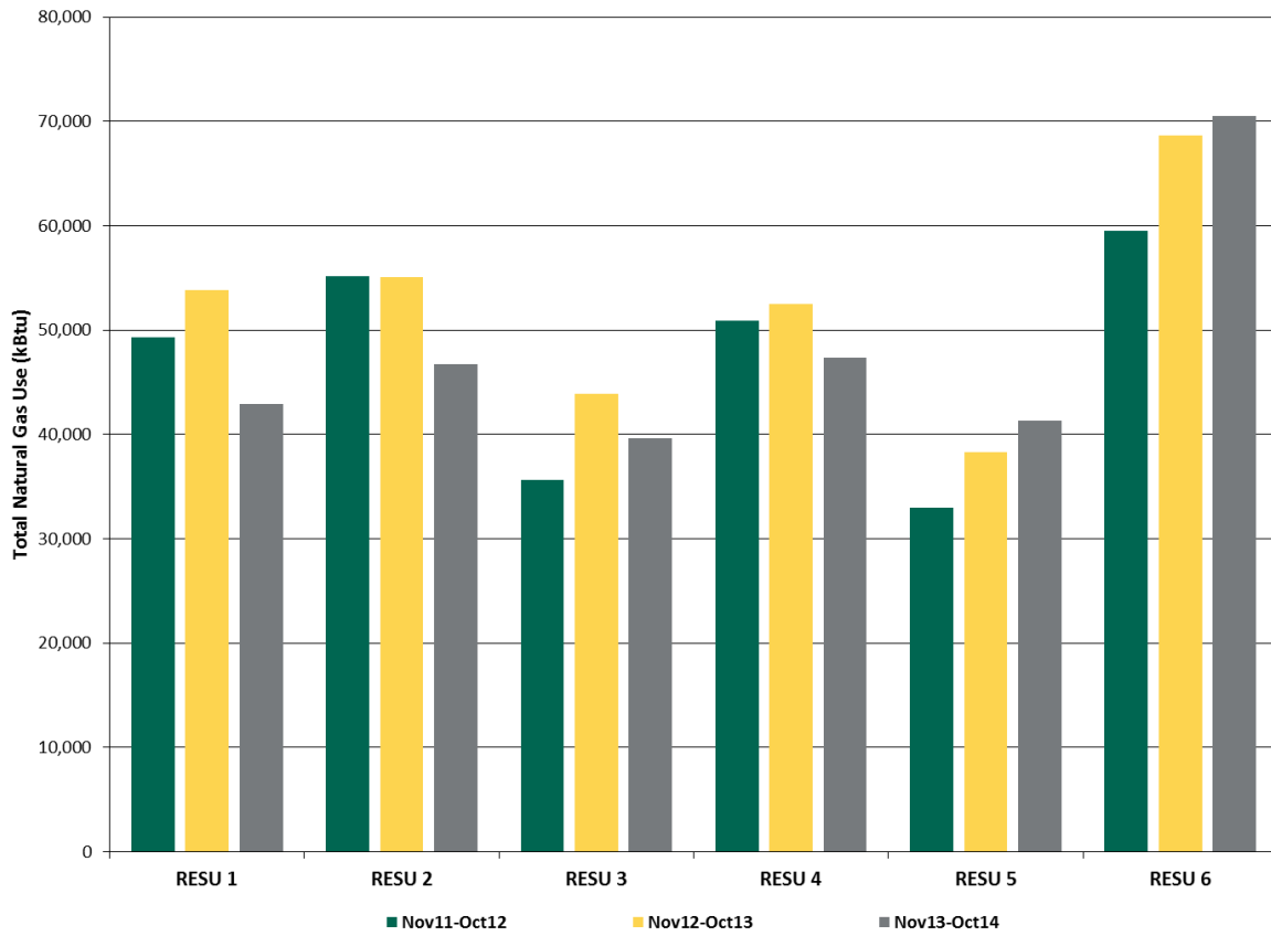
Figure 18: RESU Block Natural Gas Energy Use (November 1, 2011 to October 31, 2014)
