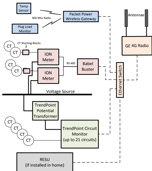
Figure 71: Home Data Collection Cabinet Block Diagram
