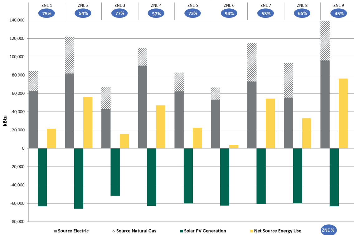
Figure 39: ZNE Source Energy Status for ZNE Block Homes (November 1, 2013 to October 31, 2014)
