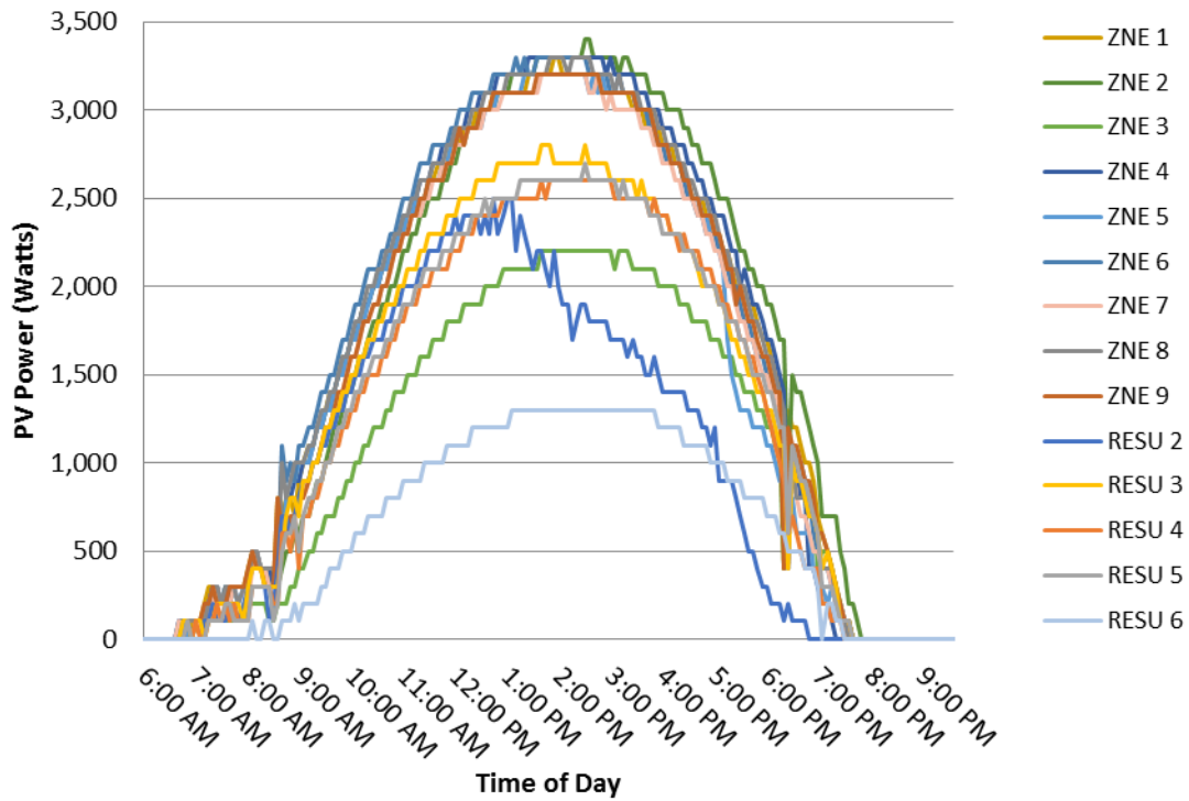
Figure 62: Solar PV Generation (June 17, 2014)
