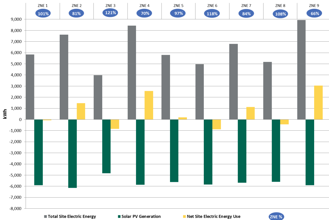
Figure 40: ZNE Site Electric Energy Status for ZNE Block Homes (November 1, 2013 to October 31, 2014)
