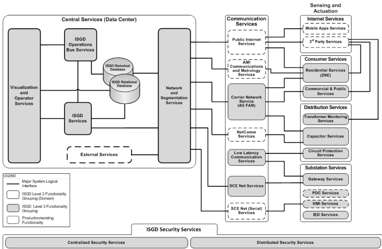
Figure 6: ISGD Logical System Architecture
