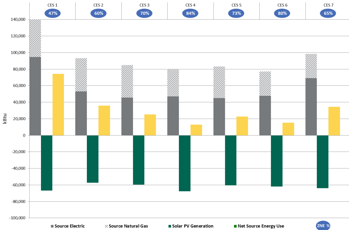
Figure 42: ZNE Source Energy Status for CES Block Homes (November 1, 2013 to October 31, 2014)
