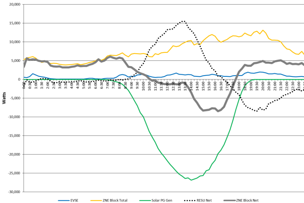
Figure 24: ZNE Block Aggregate Home Load Profile (Daily Average for September 2014)
