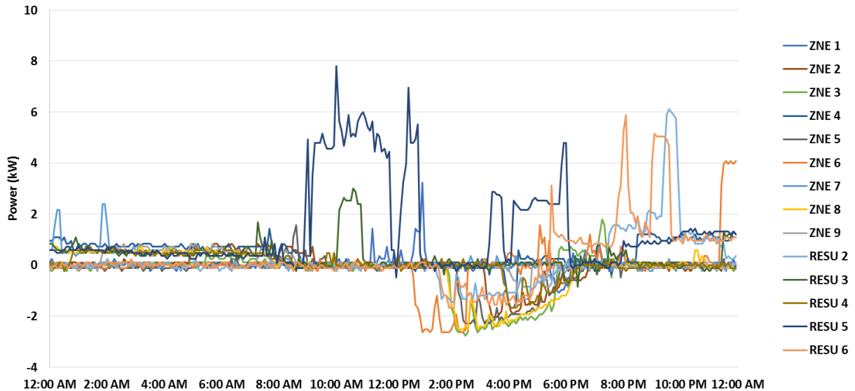
Figure 53: RESU Home Demand (July 4, 2014)
