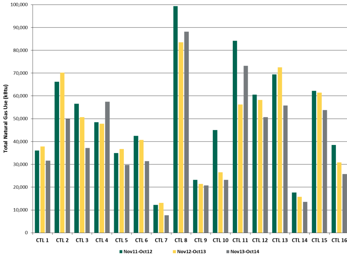
Figure 20: Control Block Natural Gas Energy Use (November 1, 2011 to October 31, 2014)
