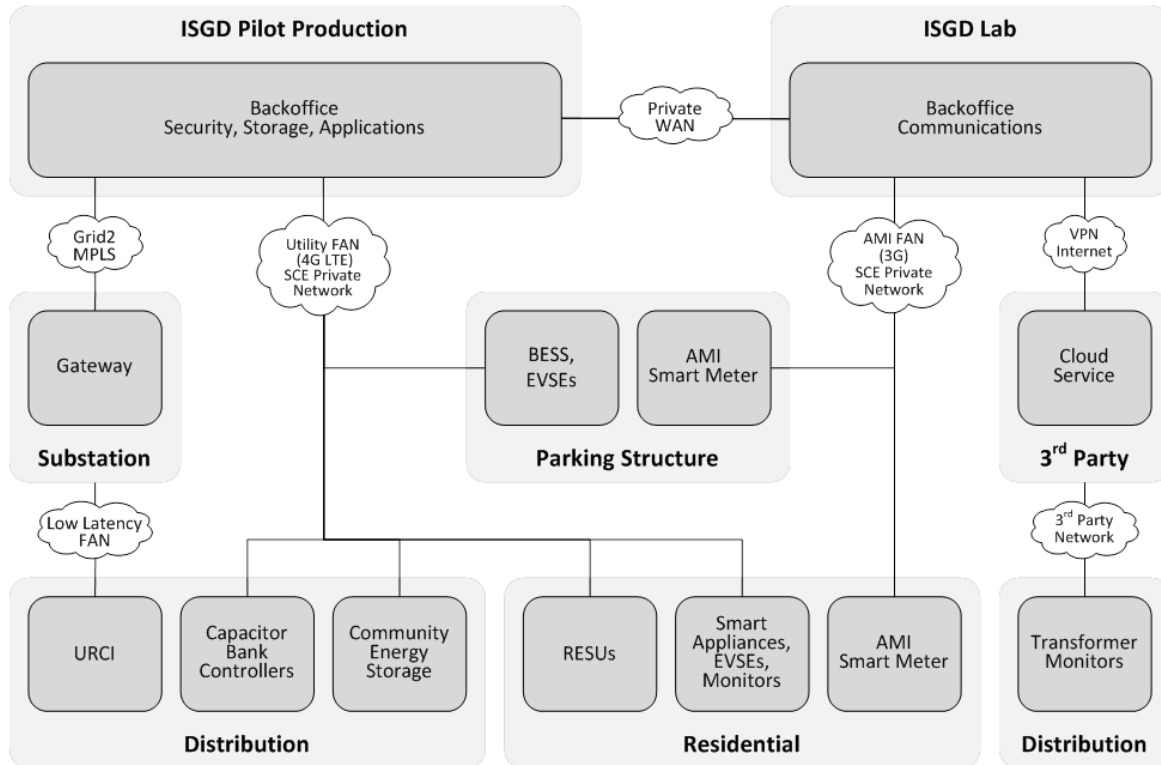
Figure 10: ISGD System Network Infrastructure Overview
