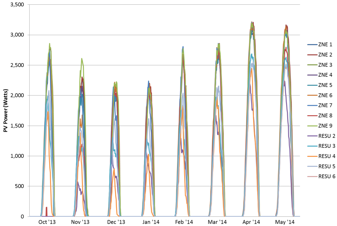
Figure 61: Average Solar PV Output (October 2013 to May 2014)
