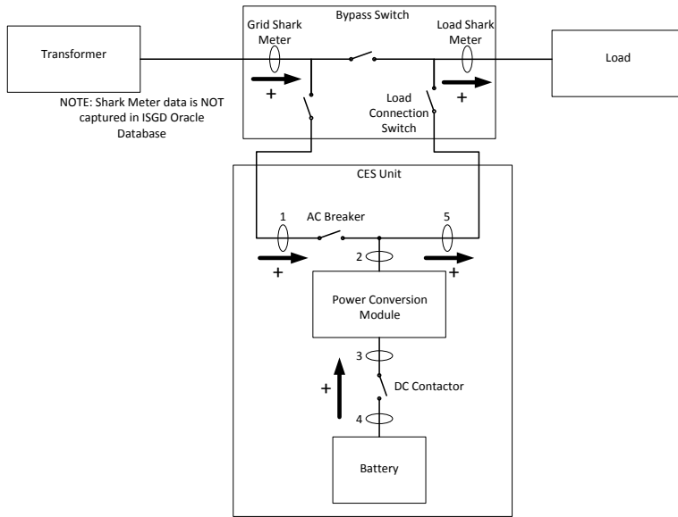
Figure 58: CES One Line Diagram
