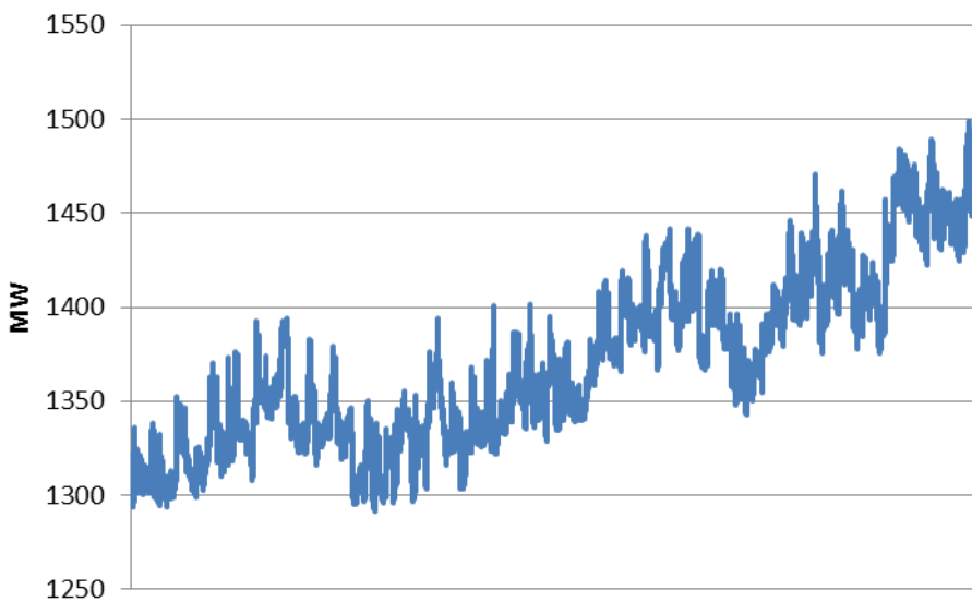
Figure 78: Rommel Circuit Real Power for One Hour Starting at 2:16:58 on 12/5/13
