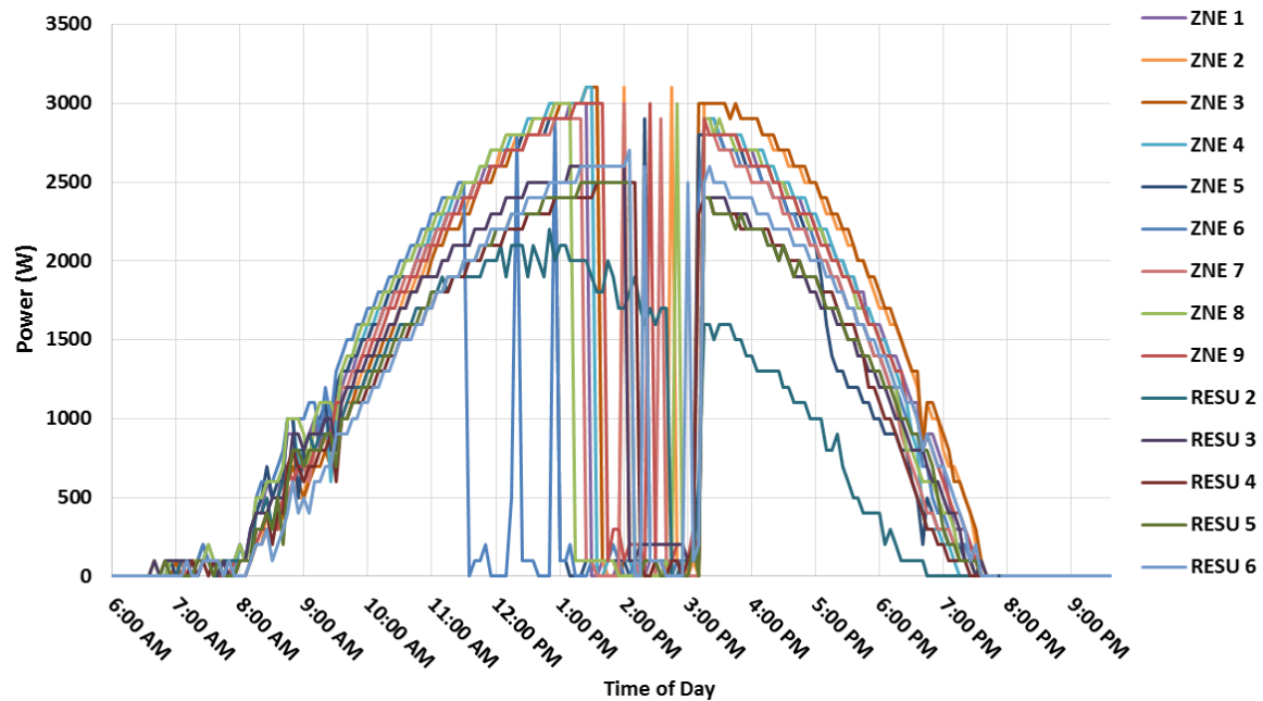
Figure 50: Solar PV Generation Output (July 8, 2014)
