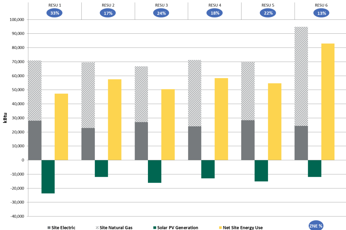
Figure 44: ZNE Site Energy Status for RESU Block Homes (November 1, 2013 to October 31, 2014)
