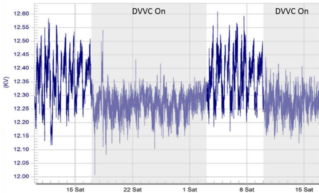
Figure 67: Substation Bus Voltages with DVVC in CVR Mode (February 15, 2014 to March 15, 2014)
