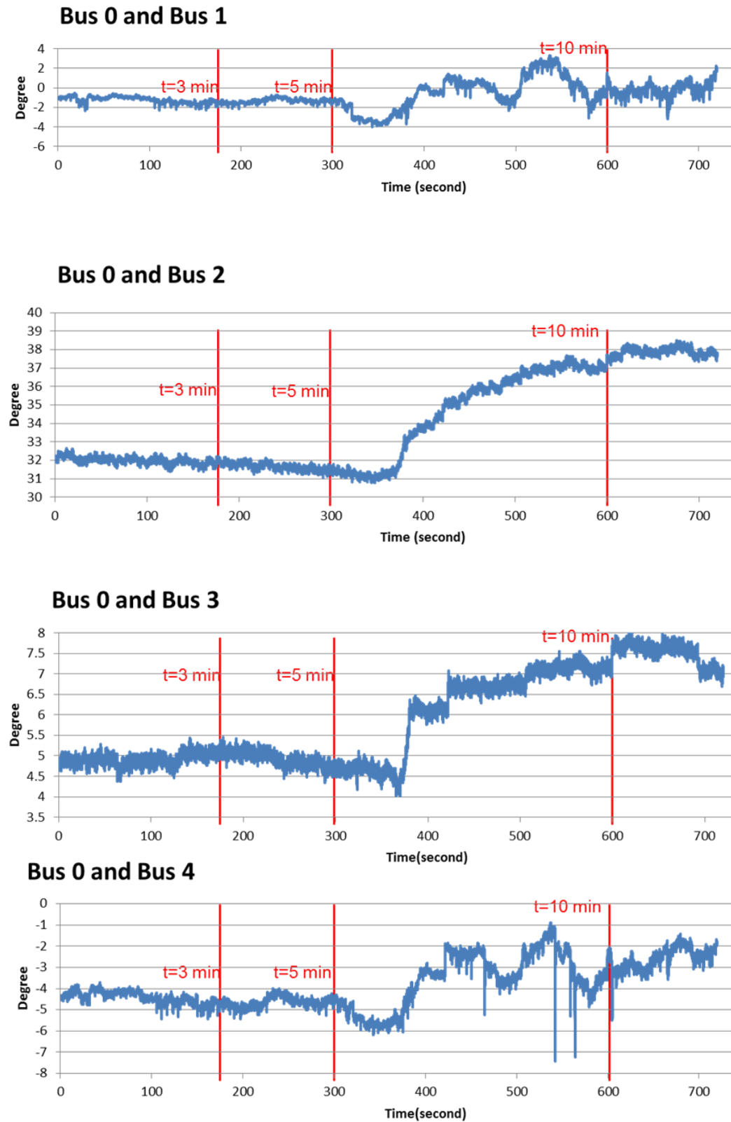
Figure 76: Phase Angle Differences between Bus 0 in Devers Substation and Adjacent Substations
