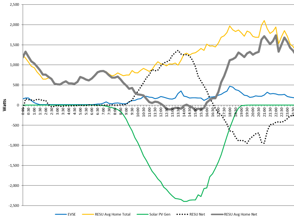
Figure 35: RESU Block Average Home Load Profile (Daily Average for September 2014)
