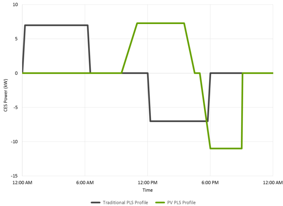
Figure 55: CES Permanent Load Shifting Profiles
