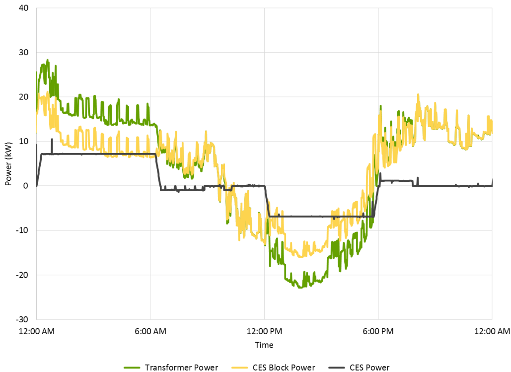
Figure 57: Load Profiles of CES, CES Block Transformer, and CES Block Load (September 19, 2014)
