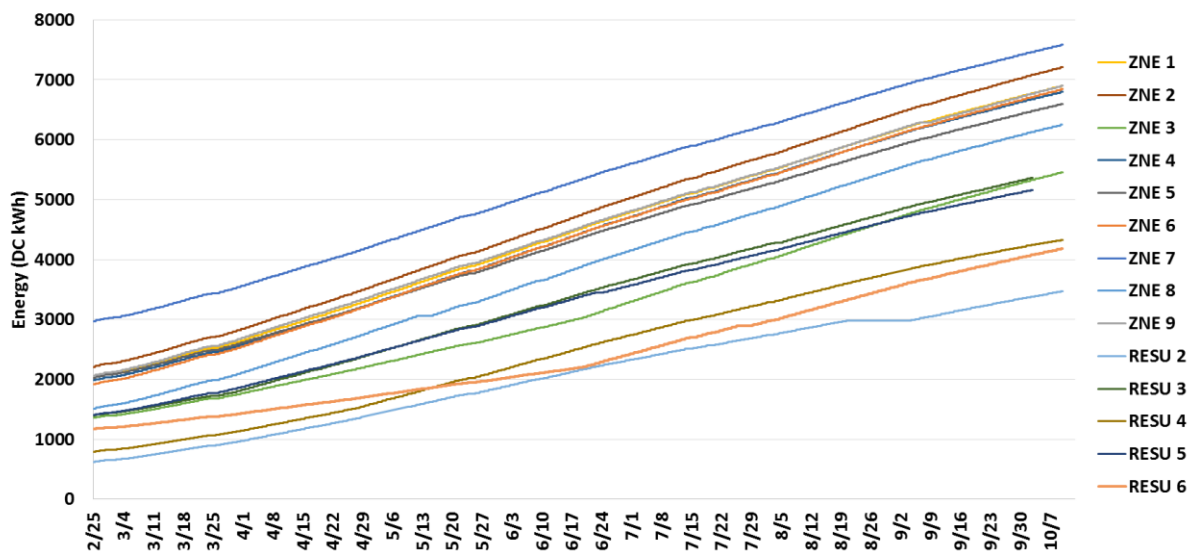
Figure 52: Cumulative Solar PV Generation
