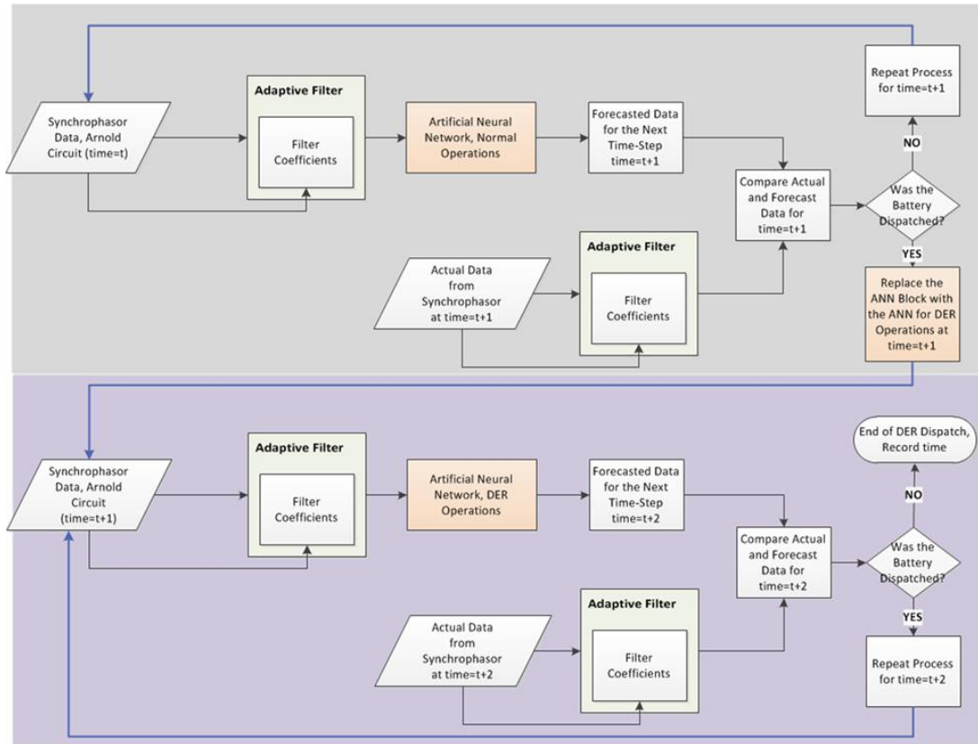
Figure 83: Overall Solution Method I
