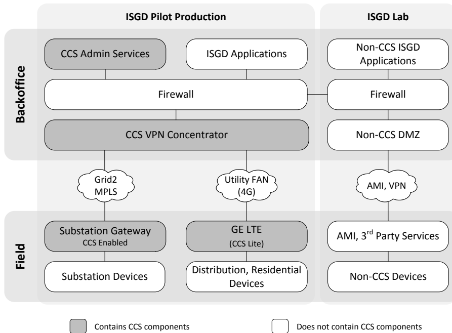
Figure 7: ISGD System Security Architecture
