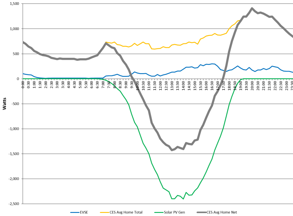
Figure 31: ZNE Block Average Home Load Profile (Daily Average for June 2014)
