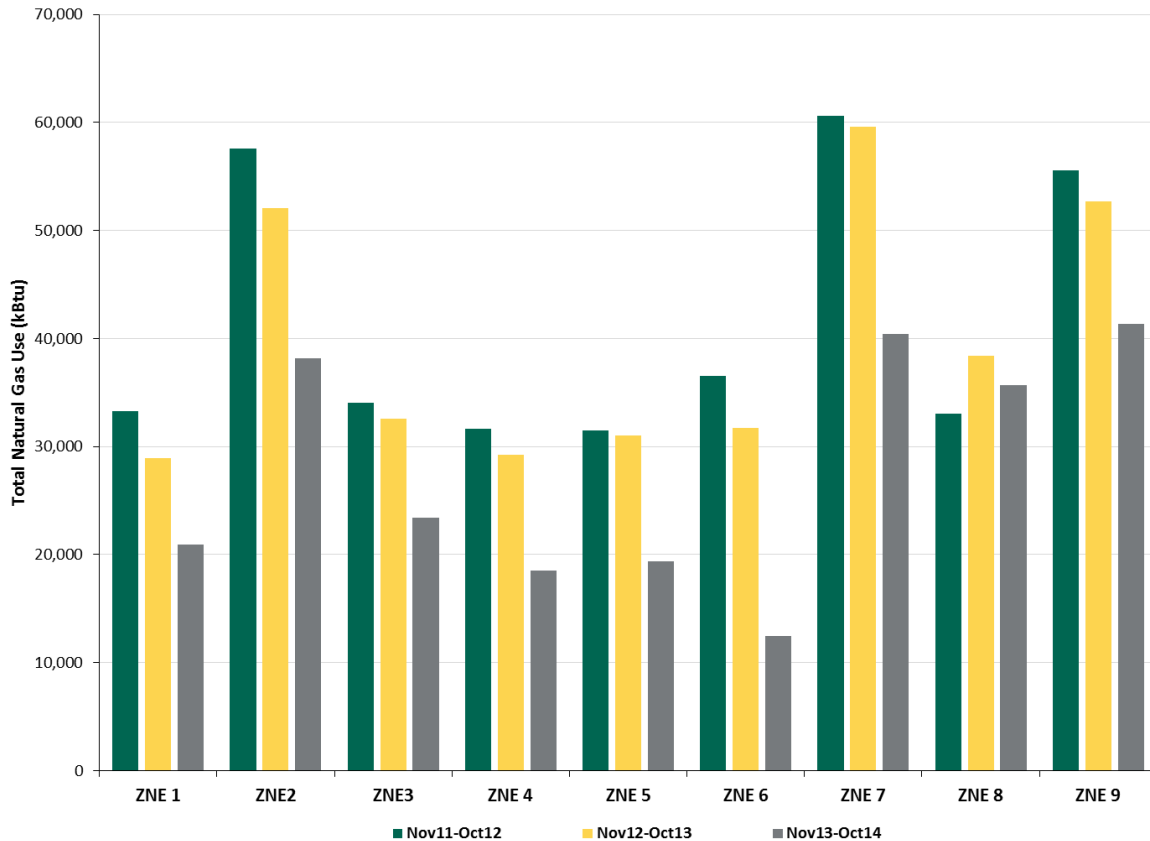
Figure 17: ZNE Block Natural Gas Energy Use (November 1, 2011 to October 31, 2014)
