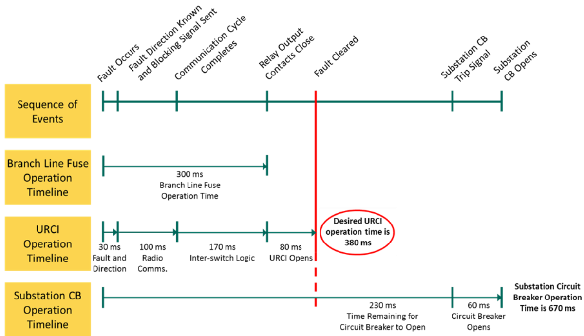
Figure 4: Distribution System Protection Event Sequence and Timeline
