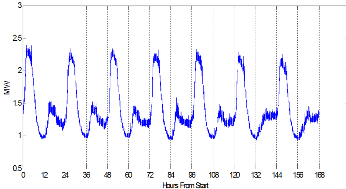
Figure 82: Arnold Circuit Real Power Starting at 4 PM (2/9/14)
