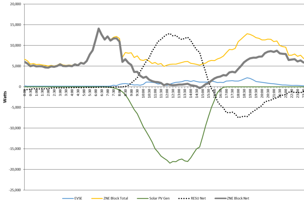
Figure 21: ZNE Block Aggregate Home Load Profile (Daily Average for December 2013)
