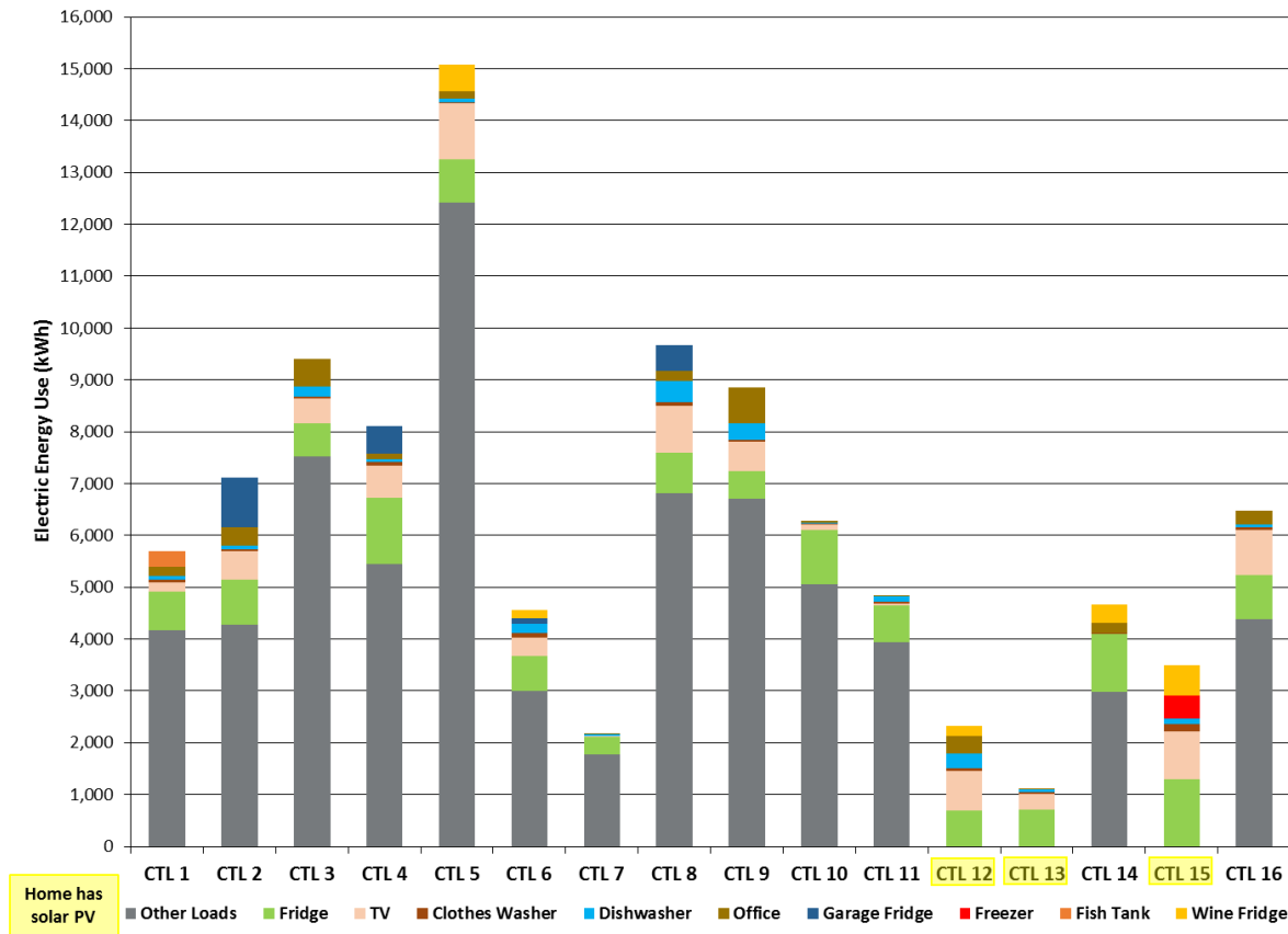
Figure 16: Control Block Electric Energy Use Breakdown (November 1, 2013 to October 31, 2014)
