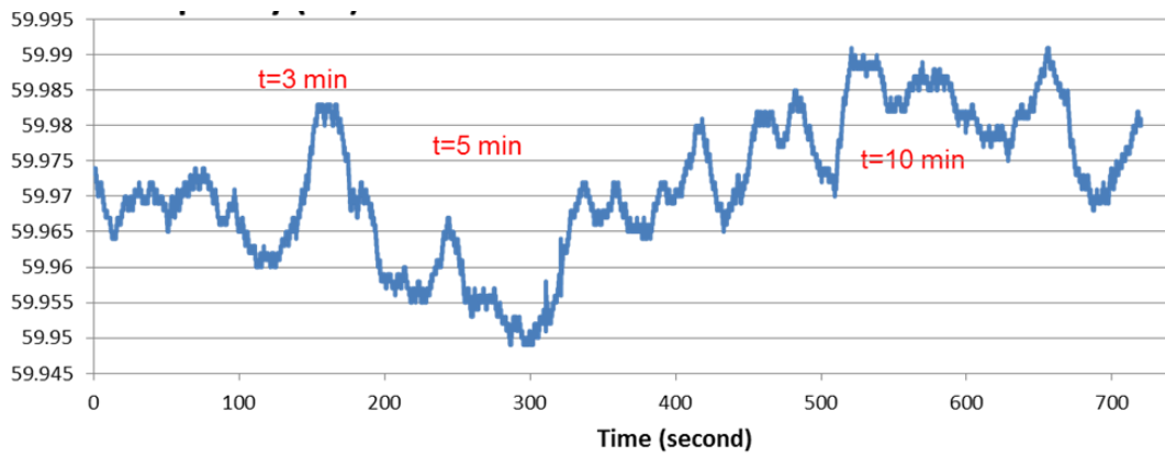
Figure 75: Frequency (Hertz)
