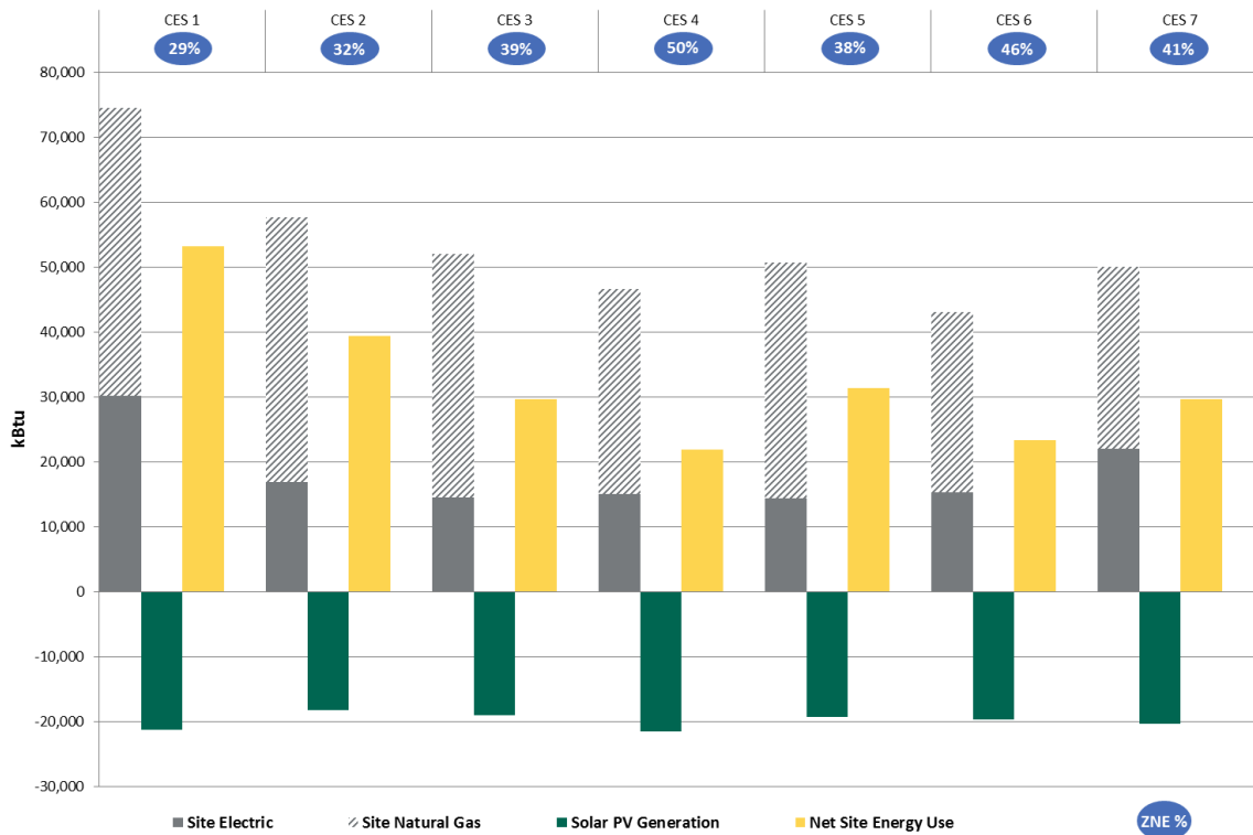
Figure 41: ZNE Site Energy Status for CES Block Homes (November 1, 2013 to October 31, 2014)
