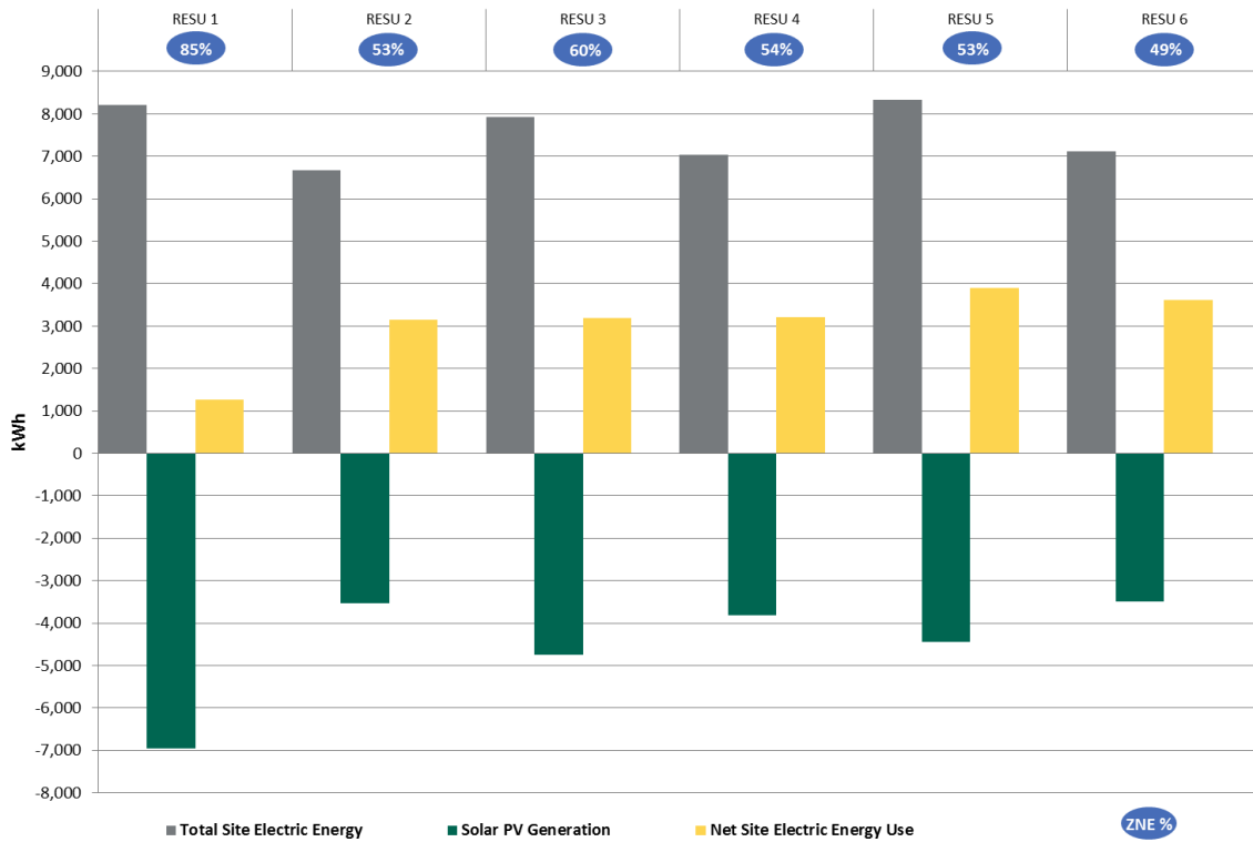
Figure 46: ZNE Site Electric Energy Status for RESU Block Homes (November 1, 2013 to October 31, 2014)
