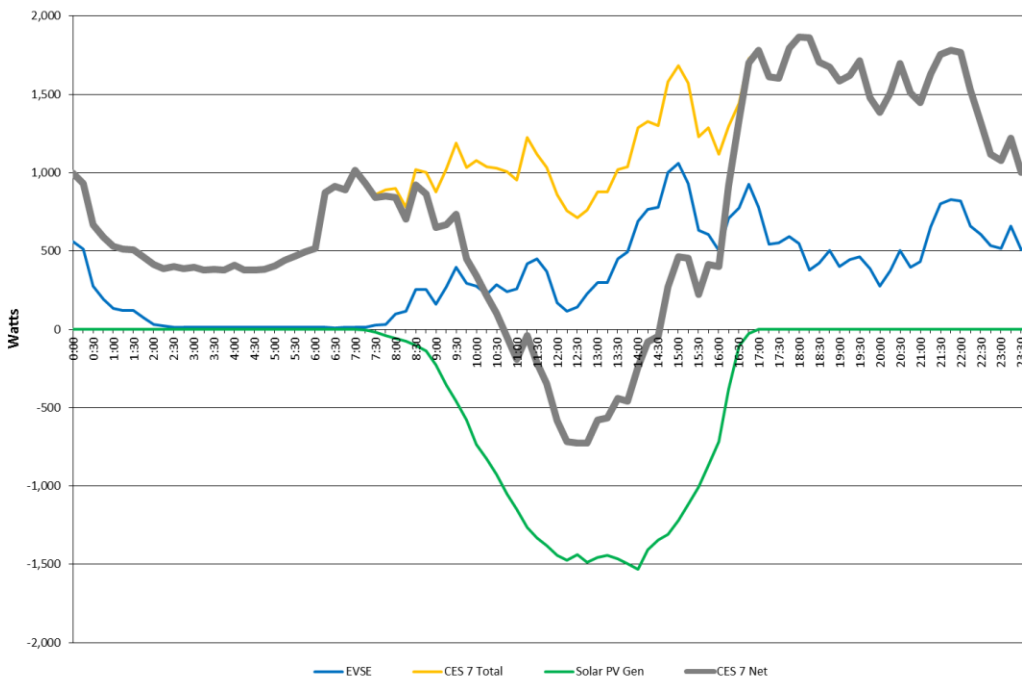
Figure 37: CES 7 Load Profiles (Daily Average for December 2013)
