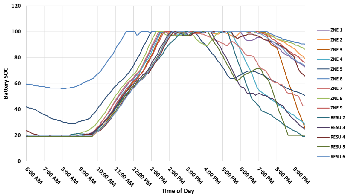
Figure 49: RESU States of Charge (July 8, 2014)
