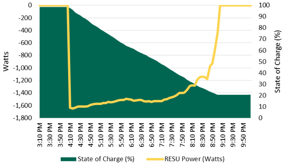
Figure 47: Average RESU Power and State of Charge (September 15, 2014)
