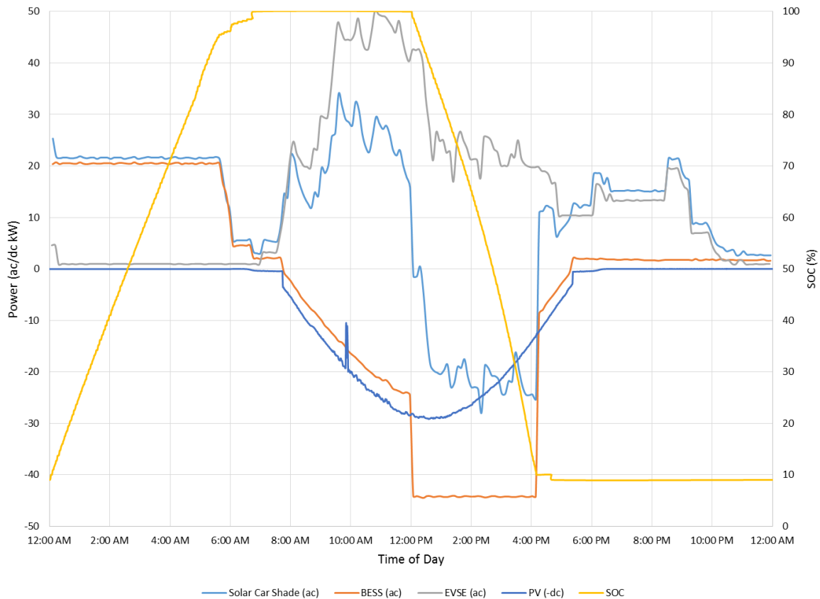
Figure 65: BESS Weekday Power Profile (October 28, 2014)
