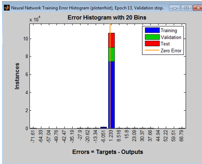
Figure 81: Error Histogram for Arnold Circuit
