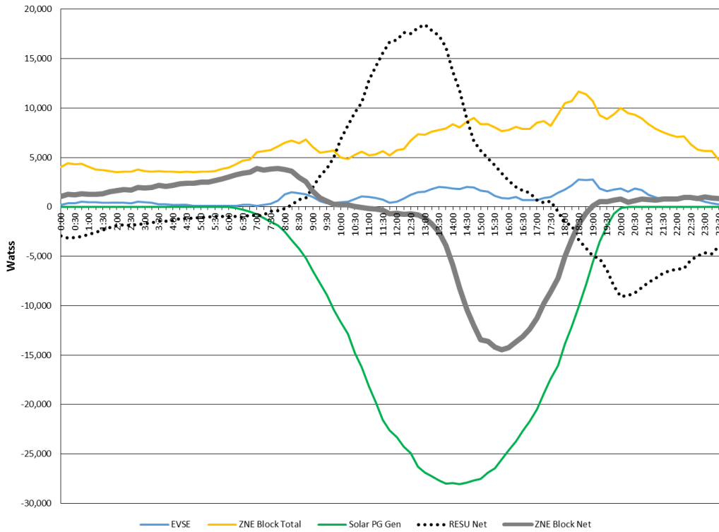
Figure 24: ZNE Block Aggregate Home Load Profile (Daily Average for September 2014)
