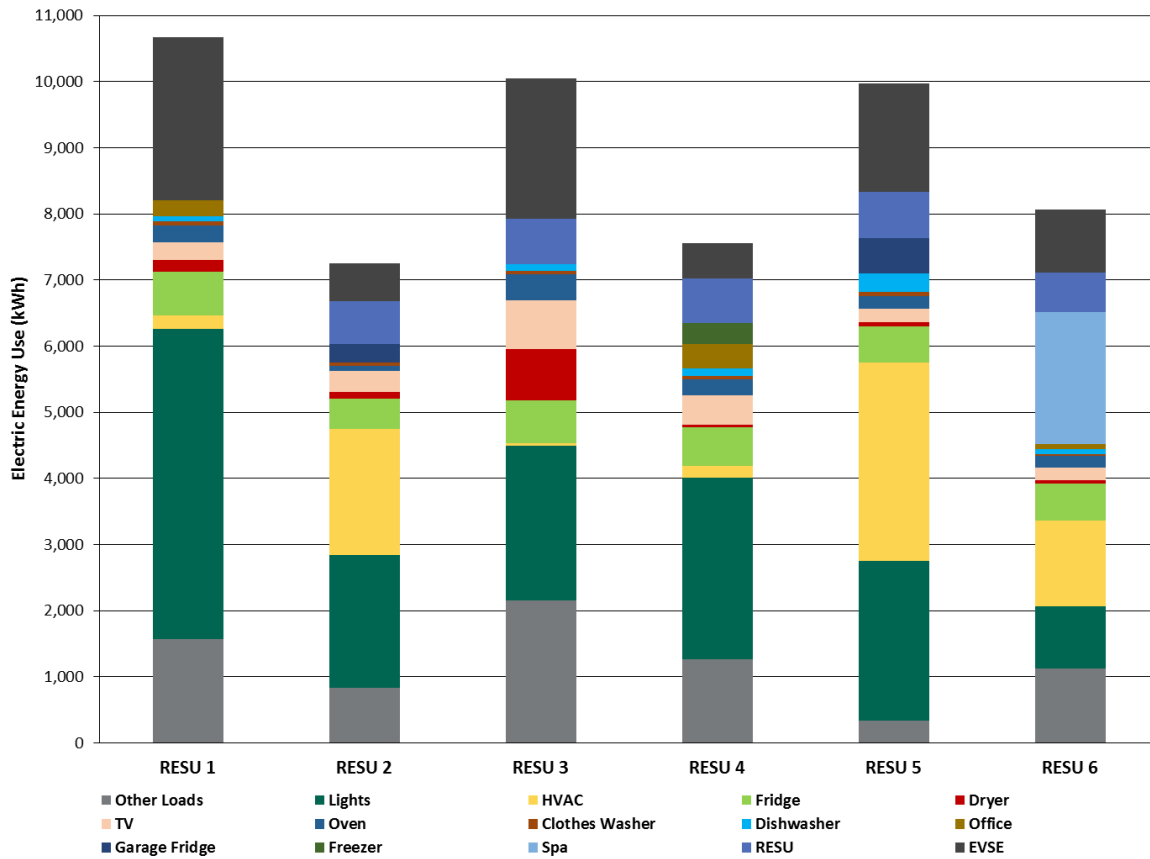
Figure 14: RESU Block Electric Energy Use Breakdown (November 1, 2013 to October 31, 2014)
