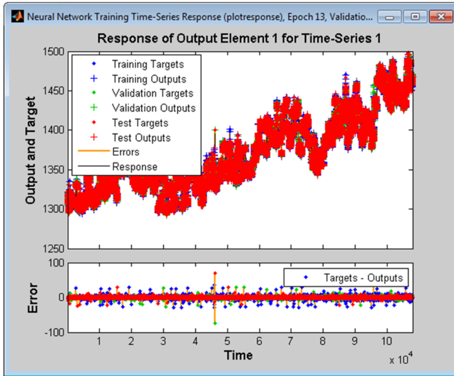
Figure 80: Neural Network Training Results for Arnold Circuit
