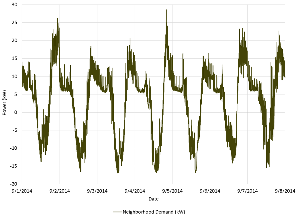
Figure 59: CES Block Load Profile (Week of September 1, 2014)
