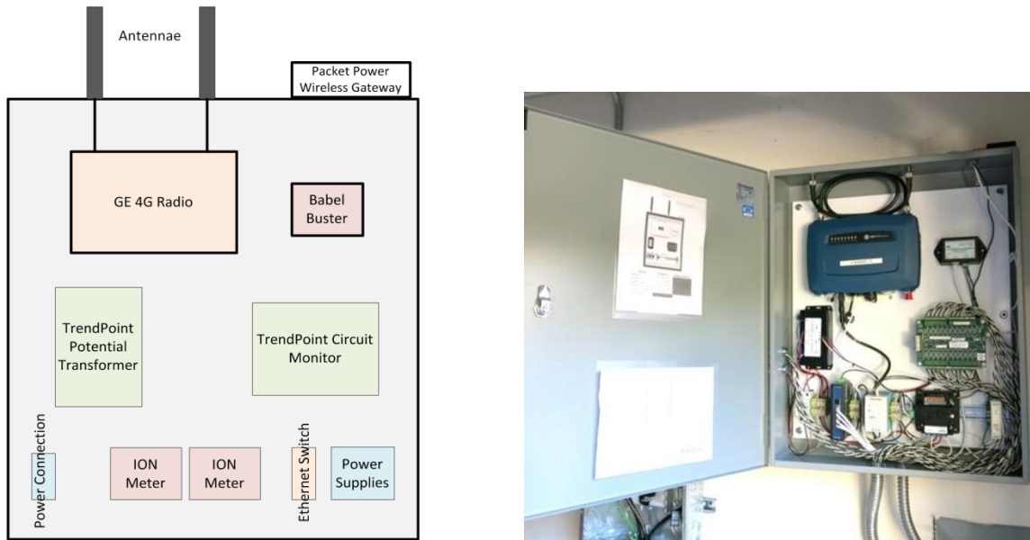
Figure 70: Home Data Collection Cabinet Arrangement
