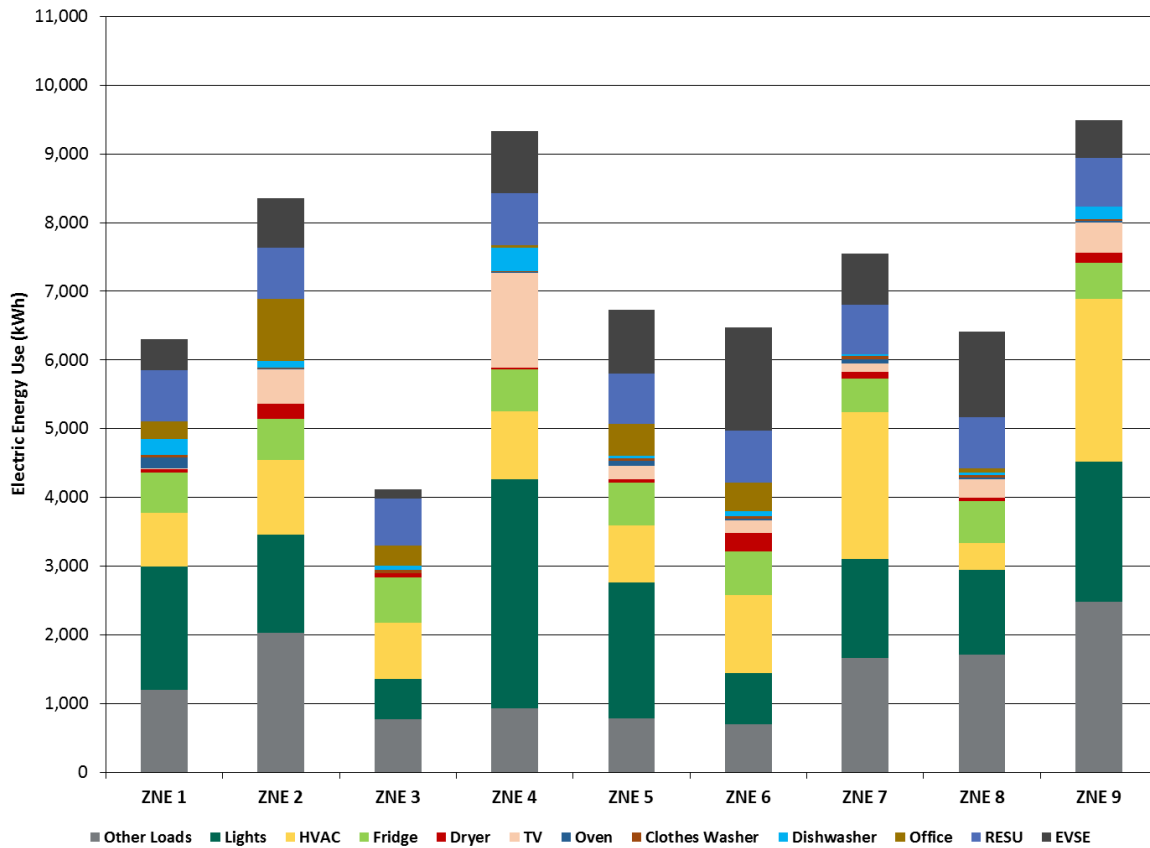
Figure 13: ZNE Block Electric Energy Use Breakdown (November 1, 2013 to October 31, 2014)
