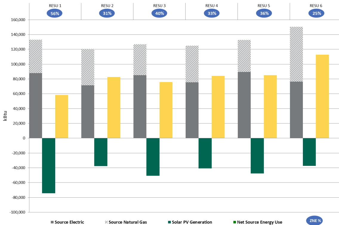
Figure 45: ZNE Source Energy Status for RESU Block Homes (November 1, 2013 to October 31, 2014)
