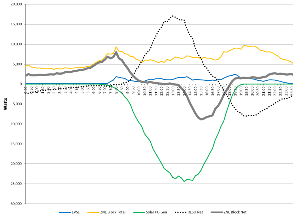
Figure 22: ZNE Block Aggregate Home Load Profile (Daily Average for March 2014)
