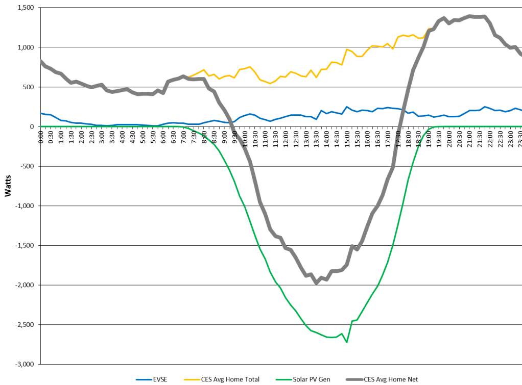
Figure 36: CES Block Average Home Load Profile (Daily Average for September 2014)
