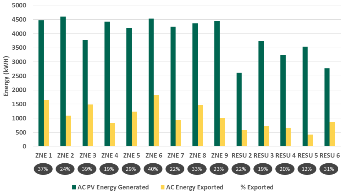
Figure 54: Solar PV Generation and Export
