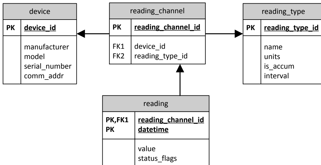
Figure 73: Reference Model Example Using an Intermediate Table
