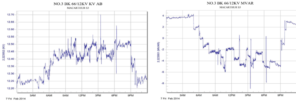
Figure 66: VAR Support Mode (February 7, 2014)
