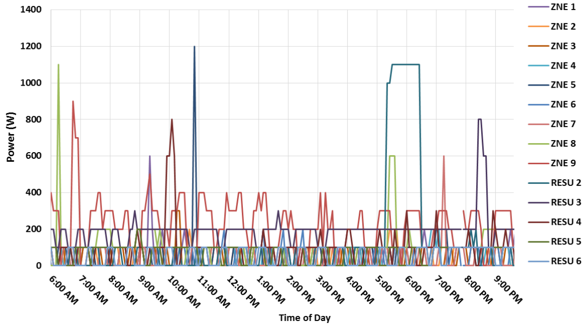
Figure 51: RESU Secure Load Power Levels During Outage (July 8, 2014)
