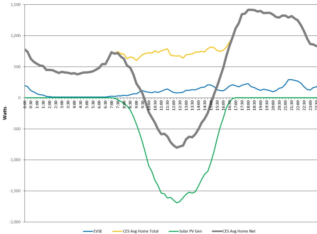
Figure 27: CES Block Average Home Load Profile (Daily Average for December 2013)
