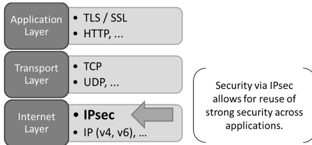
Figure 11: IPSec in the Internet Protocol Suite
