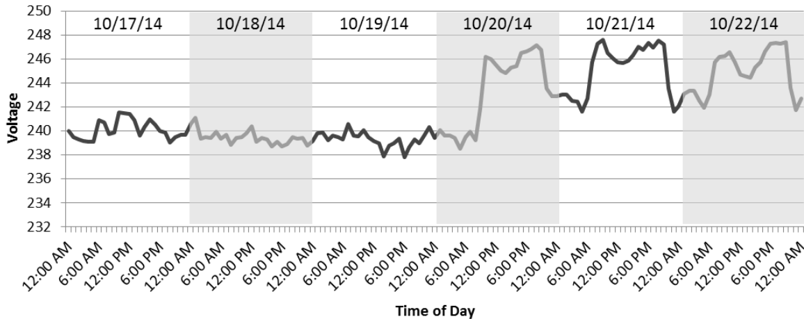
Figure 68: Customer Voltages with and without DVVC (October 17, 2014 to October 22, 2014)
